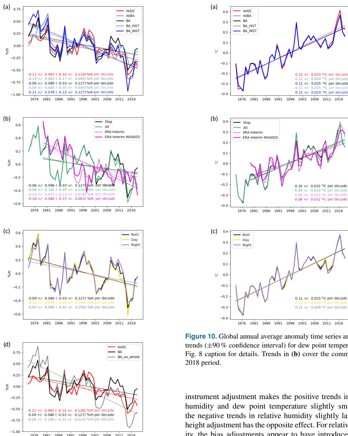
Figure 9. Global annual average anomaly time series and decadal trends ( \pm 90\% confidence interval) for relative humidity. See Fig. 8 caption for details. In addition, panel (d) shows the time series from the bias-adjusted data with removal of any data with a whole-number flag set (BA_no_whole). Trends in (b) cover the common 1979–2018 period, and all trends in parentheses cover the 1982–2018 period.
